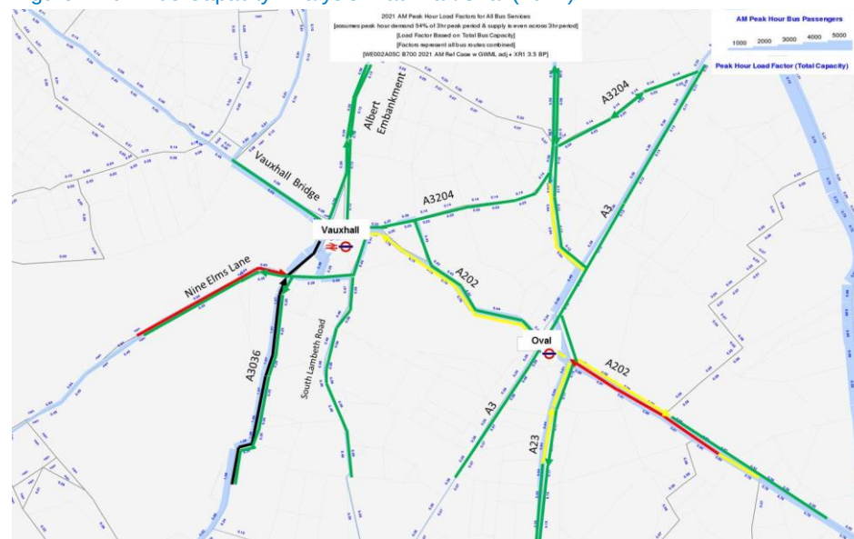
Figure 4.10: Bus Capacity Analysis: Vauxhall/Oval (2021)
