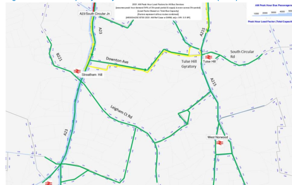
Figure 4.15: Bus Capacity Analysis: Streatham/West Norwood (2031)
