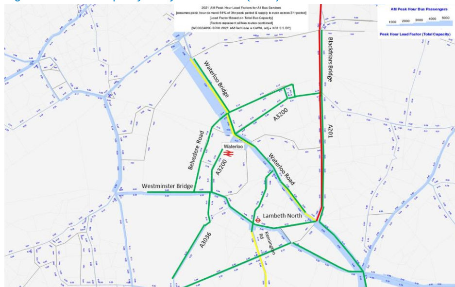
Figure 4.8: Bus Capacity Analysis: Waterloo (2021)
