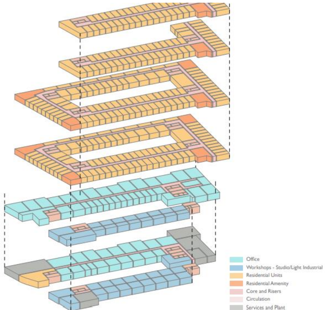
Exploded Axonometric
